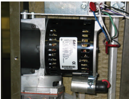
Gast Pump Model 74R142-V122-H203X Fig A
